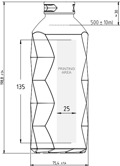
Pogled z desne Right view
