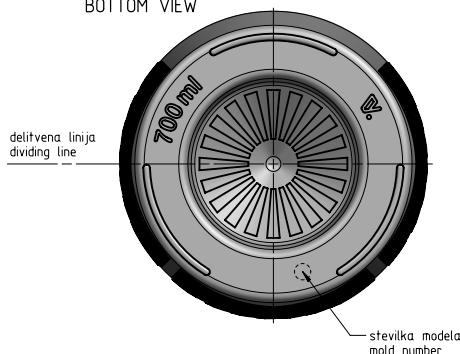
POGLED DOL BOTTOM VIEW
